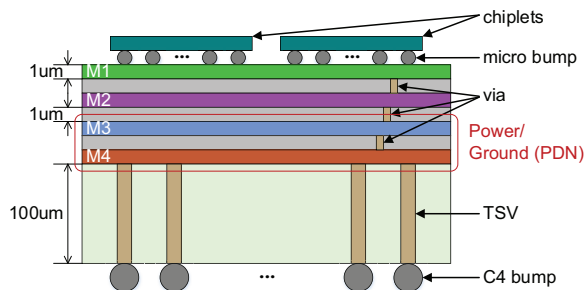
Figure 4: Vertical stack-up of our interposer-based 2.5D IC.
