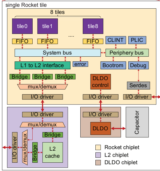
Figure 2: Our proposed 64-core architecture for chipletization and 2.5D integration.
