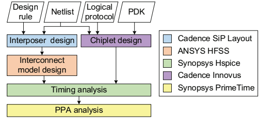
Figure 3: Our EDA flow using commercial tools.
