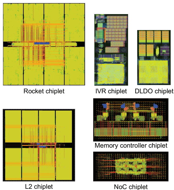
Figure 6: Commercial 28nm and 130nm physical layouts of the chiplets in our ROCKET-64 architecture (not drawn in scale). The blue part shows protocol translator/bridge logic.
